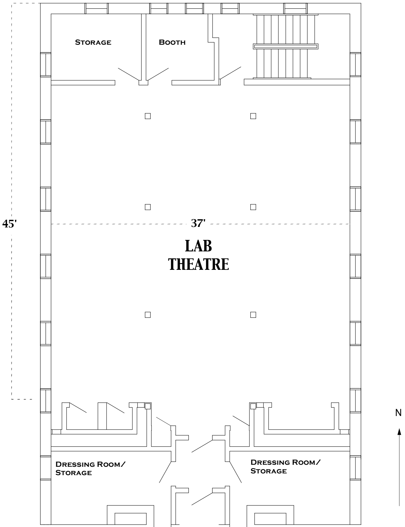
THERE ARE 6 STRUCTURAL PILLARS IN THE LAB THEATRE DRAWING IS NOT TO SCALE.
